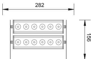
LED3*ADJ DOUBLE STRIP 6 CODE: LADS06 12xLED
